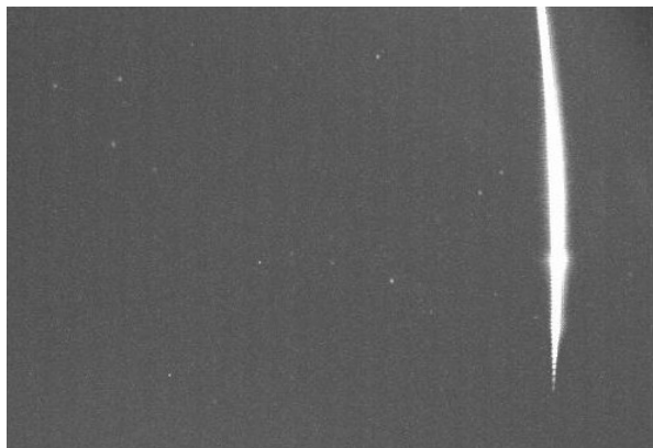
Figure 3. Composite image of a -10 magnitude October Capricornid bolide associated with a large meteoroid from disintegrated comet D/1978 R1 Haneda-Campos. Recorded from Folgueroles station on Oct. 12 th 2011 at 22h45m27.3s UTC (SPMN 121011). Cassiopeia, and Perseus constellations are easily identifiable constellations.
