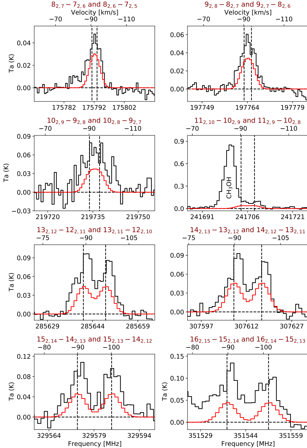
Figure 4. As in the caption of Fig. 1. HNC0 emission lines ( K_a = 2 ) and their LTE models. The transitions are indicated in the top left corner of each plot.
