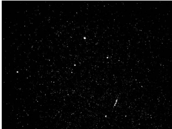
Figure 2. Trace of a SPO meteor on a registered and stack image. The brightest star is Beta Peg.
