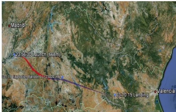
Figure 3. Ground track of the probe through Spain. Total length of 210 km (In red the data. In blue, the model).
