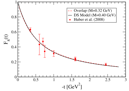
Fig. 1. Pion's electromagnetic form factor expressed by Eq. (28) (dashed red line), with the model mass parameter fixed by Eq. (30) and displayed in terms of -t in GeV, compared to experimental data [52] (red solid circles) and to the results obtained in Ref. [28] within a covariant DS-inspired calculation (black solid line) where a different model mass parameter, M = 0.40 GeV, was determined. (For interpretation of the colours in the figure(s), the reader is referred to the web version of this article.)
