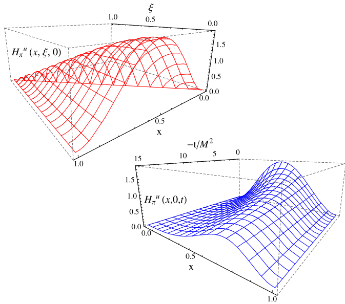
Fig. 2. DGLAP GPD given by Eq. (24) and obtained from the overlap of LFWFs, Eqs. (21)–(22), expressed by Eq. (23), plotted in terms of x and \xi , at t = 0 (upper panel); and in terms of x and t at \xi = 0 (lower panel).
