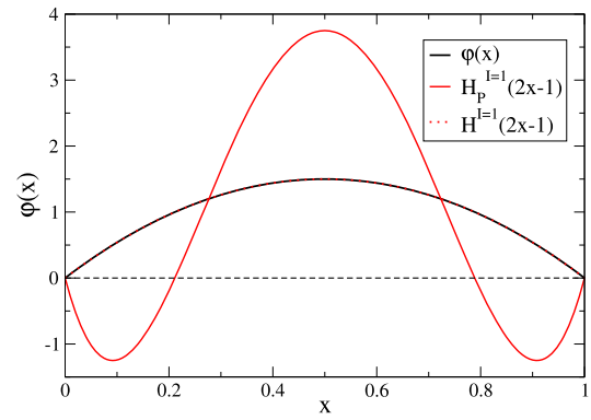
Fig. 3. Check of the soft pion theorem. H_p^{I=1}(2x-1, 1) (red solid line), the maximally skewed GPD with D^+(\alpha, 0) \equiv 0 , clearly differs from the asymptotic pion's distribution amplitude, \varphi(x) (black solid line). Only after incorporating the term D^+(\alpha, 0) given by (37) do H^{I=1}(2x-1, 1) (red dotted line) and \varphi(x) agree with each other, as dictated by Eq. (10).
