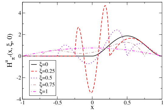
Fig. 4. The full GPD at t = 0 , expressed by Eq. (6), where H_{P_{\pi^+}}^u is given by Eq. (24) for DGLAP and by Eq. (35) for ERBL, and D^- and D^+ appear constrained by Eq. (36) and Eq. (37), respectively. The results displayed stand for \xi = 0, 0.25, 0.5, 0.75 and 1.
