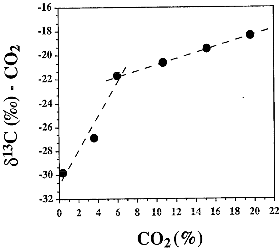
Fig.3 Relationship between soil gas CO 2 concentrations and \delta^{13}\text{C}-\text{CO}_2 from Rabaul caldera. Dashed lines represent two different trends.
